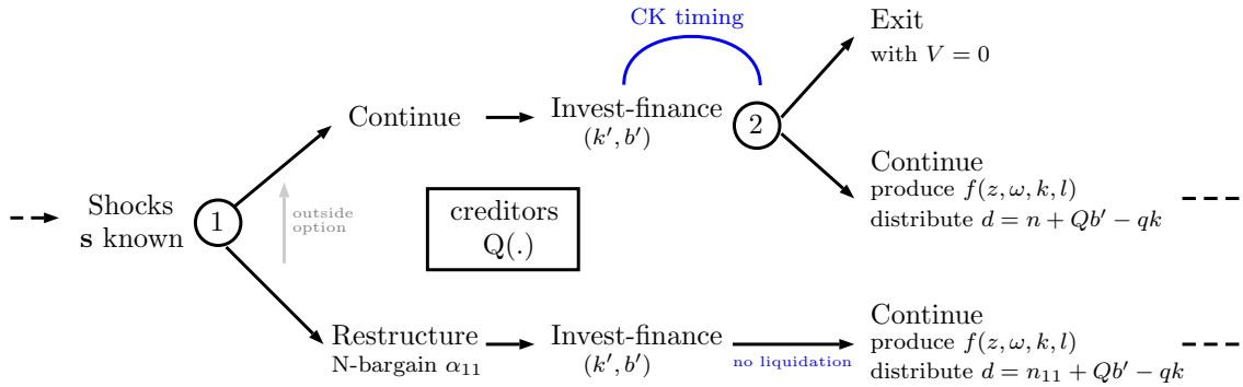
Figure 1: Within-period timing
